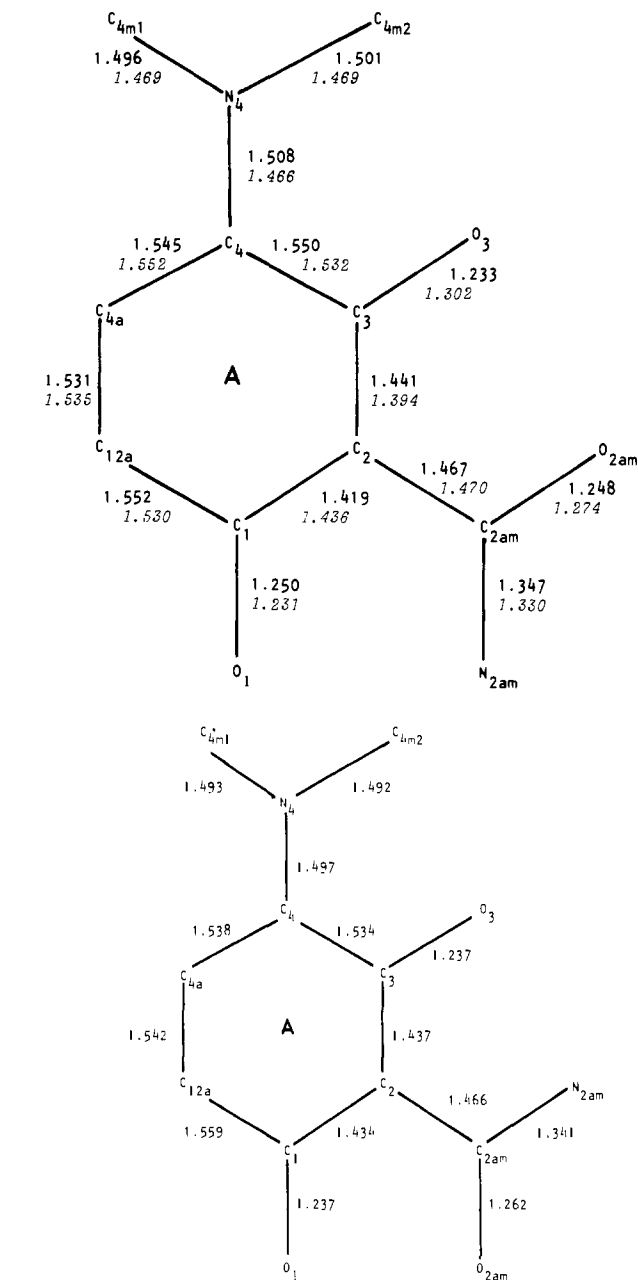
Figure 2. A-ring bond distances. The observed bond distances for zwitterionic oxytetracycline free base (normal type) and the average bond distances from nonionized oxytetracycline and diacetyloxytetracycline free bases (italicized) are presented in 2a (top). Similarly, 2b (bottom) displays the bond distances for zwitterionic tetracycline free base.
